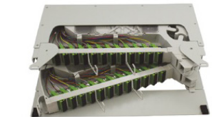
19" 2 UNITS
